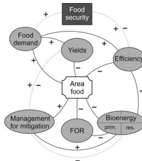
Fig. 2 Interrelationships between different bundles of GHG mitigation options (grey shaded boxes) and food security. Area for food production (food area) is a central link of the system. Option bundles refer to changing food demand, increasing yields in agriculture, increasing efficiency in the food supply chain, including livestock feeding efficiency, mitigation options related to cropland management (e.g. no-tillage agriculture), reduced deforestation, peatland conversion or afforestation (forest area) and bioenergy production, either from primary or secondary biomass sources (e.g. residues). '+' and '-' indicate the direction of the interrelationship: '+' indicates that growth of one factor drives up another; note that mitigation options related to food demand would reduce losses or resource-intensive food (e.g. animal products) which would also reduce food area, but might have feedbacks on yields and efficiency. Dotted lines indicate ambiguous or loose interrelationships.
